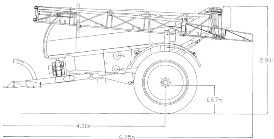
4000L with 24m boom and standard drawbar
